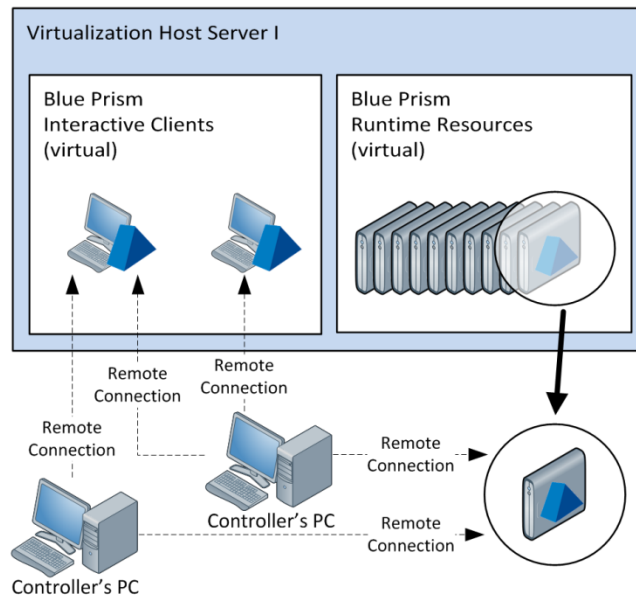
Figure 1: Example of Remote Access Connectivity to a subset of Blue Prism Resources
